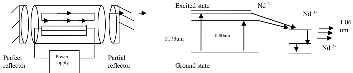
Fig.3 Constructional details and energy level diagram
