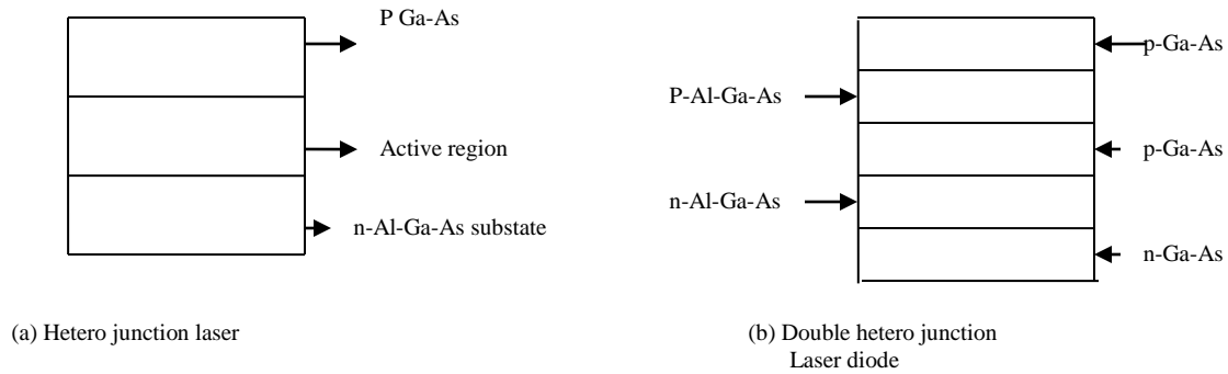
Fig.8 Hetero junction Semi conductor laser diode
