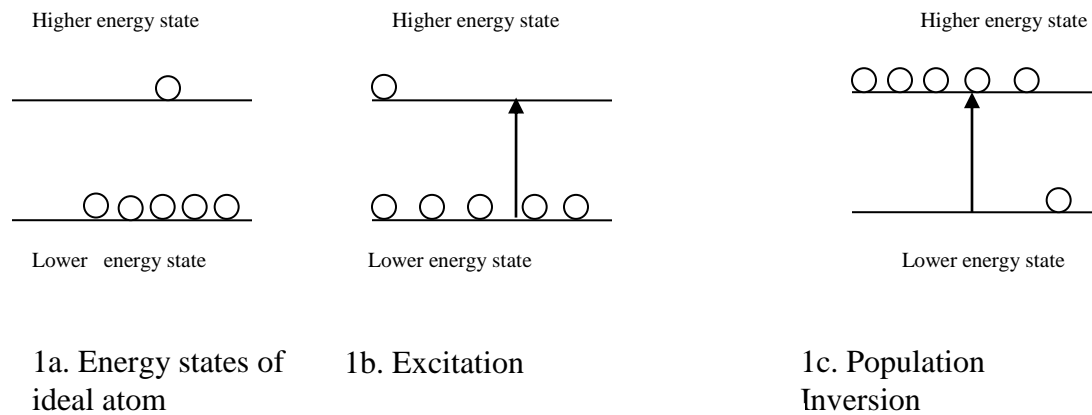
Fig.1 Ideal, Excitation and Population Inversion of atom
