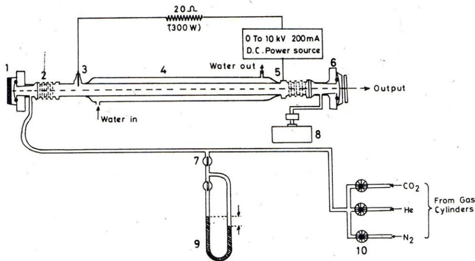
1-Perfect reflector,2-Metal bellow,3-tungtant anode,4glass jacket,5-copper cathode,6-output relector,7-glass stop cock,8-mechanical pump,9-oil monometer,10-Needle valve
