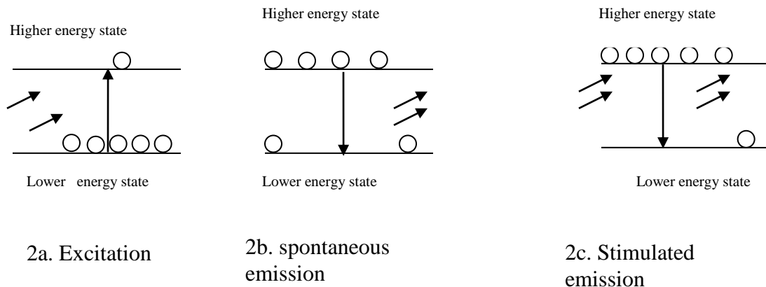
Fig.2 Excitation, spontaneous and stimulated emission
